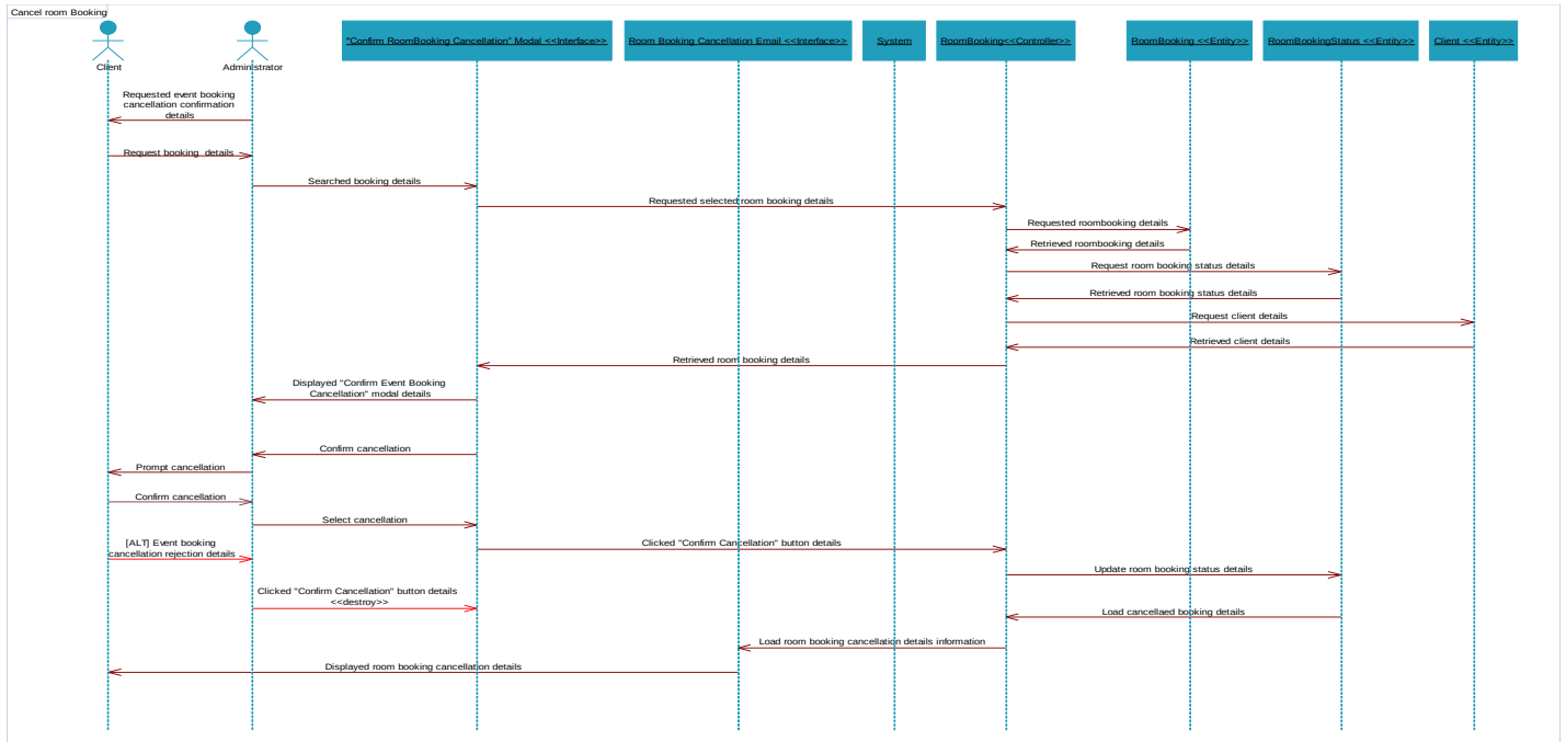
Figure 14:3.3-Cancel Room Booking Sequence Diagram
