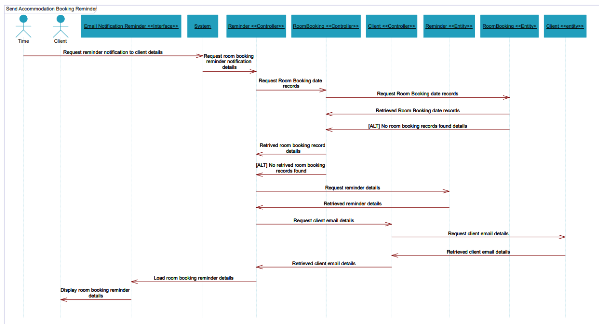
Figure 15:3.4-Send Accommodation Reminder Sequence Diagram
