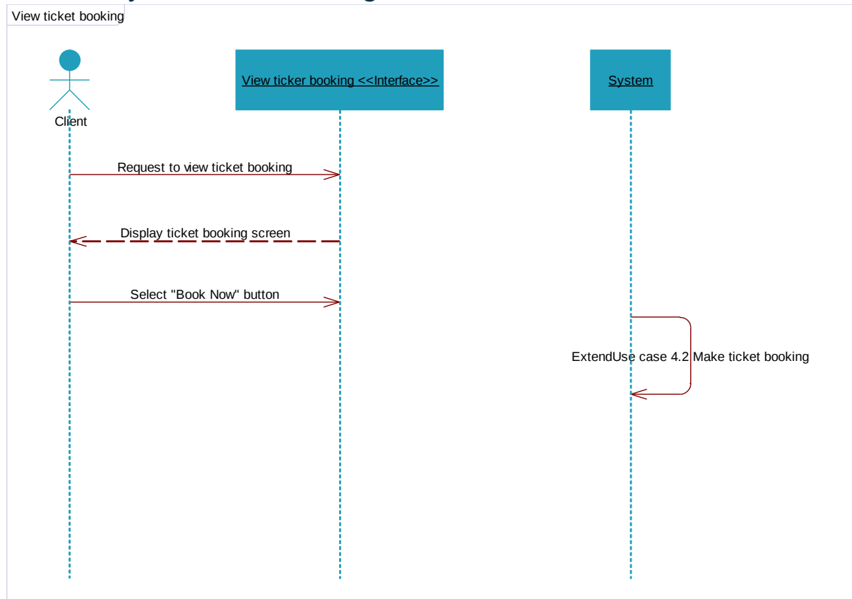
Figure 20:4.1-View Ticket Booking Sequence Diagram
