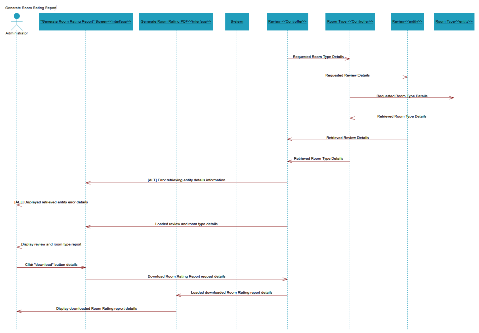
Figure 80:8.4-Generate Room Rating Report Sequence Diagram
