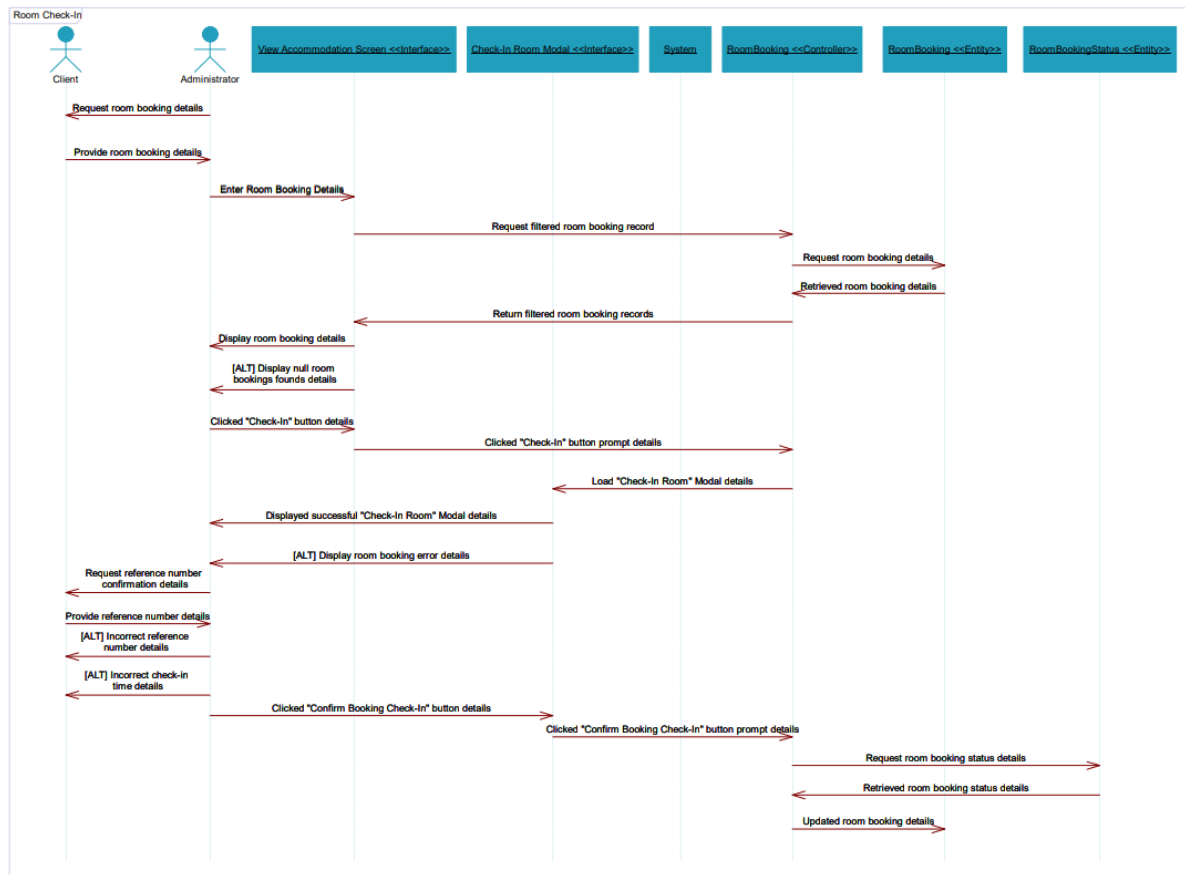
Figure 39:6.10-Room Check-In Sequence Diagram
