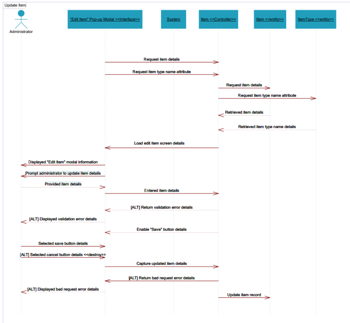
Figure 59: 7.3 Update Item Sequence Diagram
