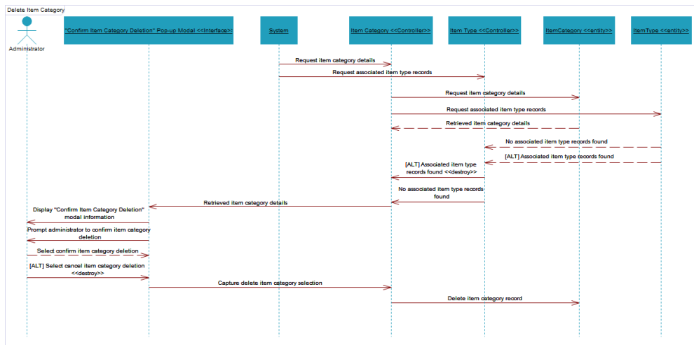
Figure 68:7.12-Delete Item Category Sequence Diagram
