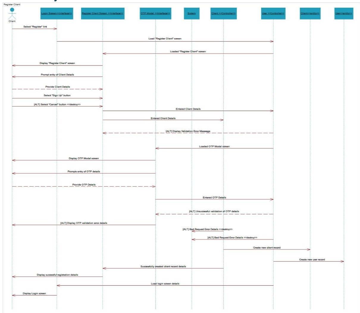
Figure 6:2.1-Register Client Sequence Diagram
