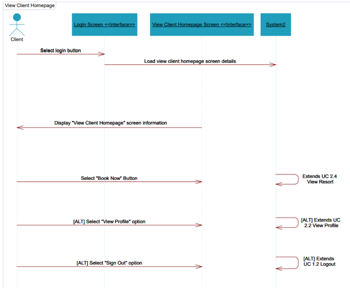
Figure 11:2.6-View Client Homepage Sequence Diagram
