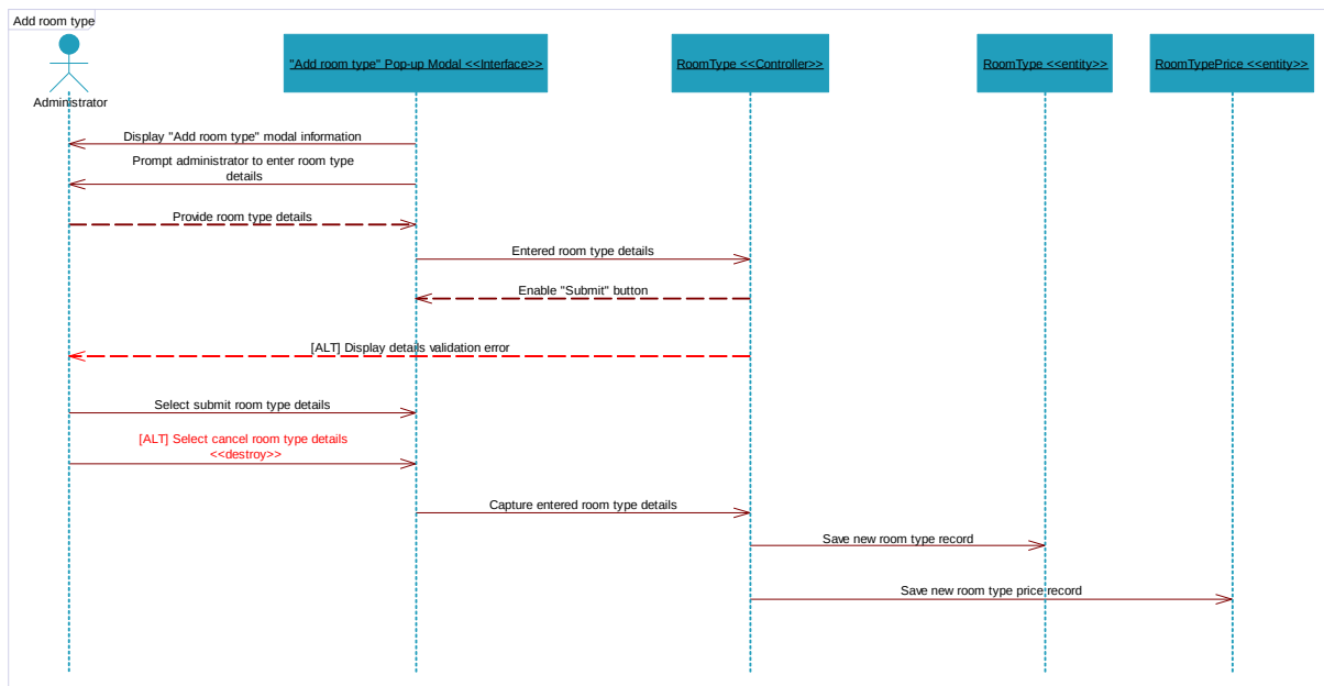
Figure 17: 3.6-Add Room Type Sequence Diagram
