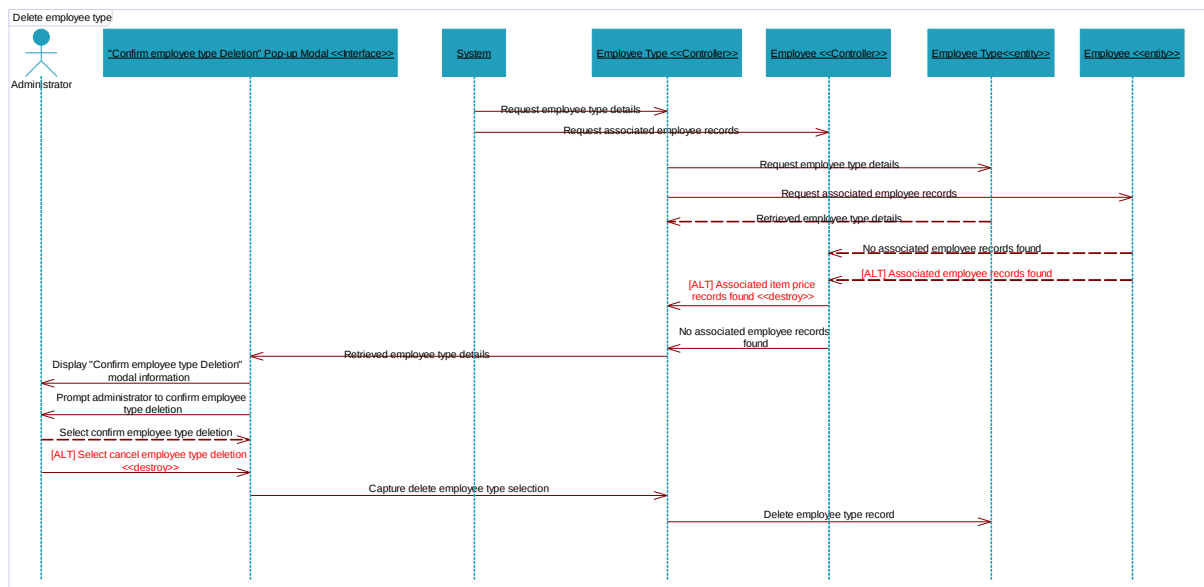
Figure 37: 6.8-Delete Employee Type Sequence Diagram
