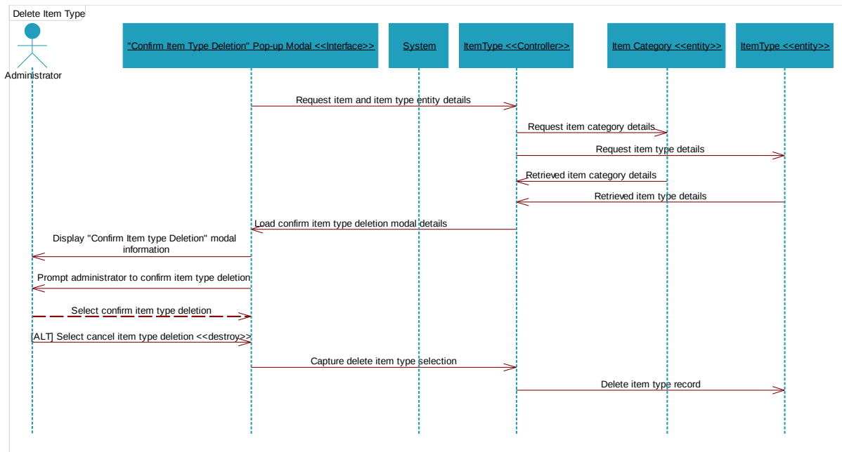
Figure 64.7.8- Delete Item Type Sequence Diagram
