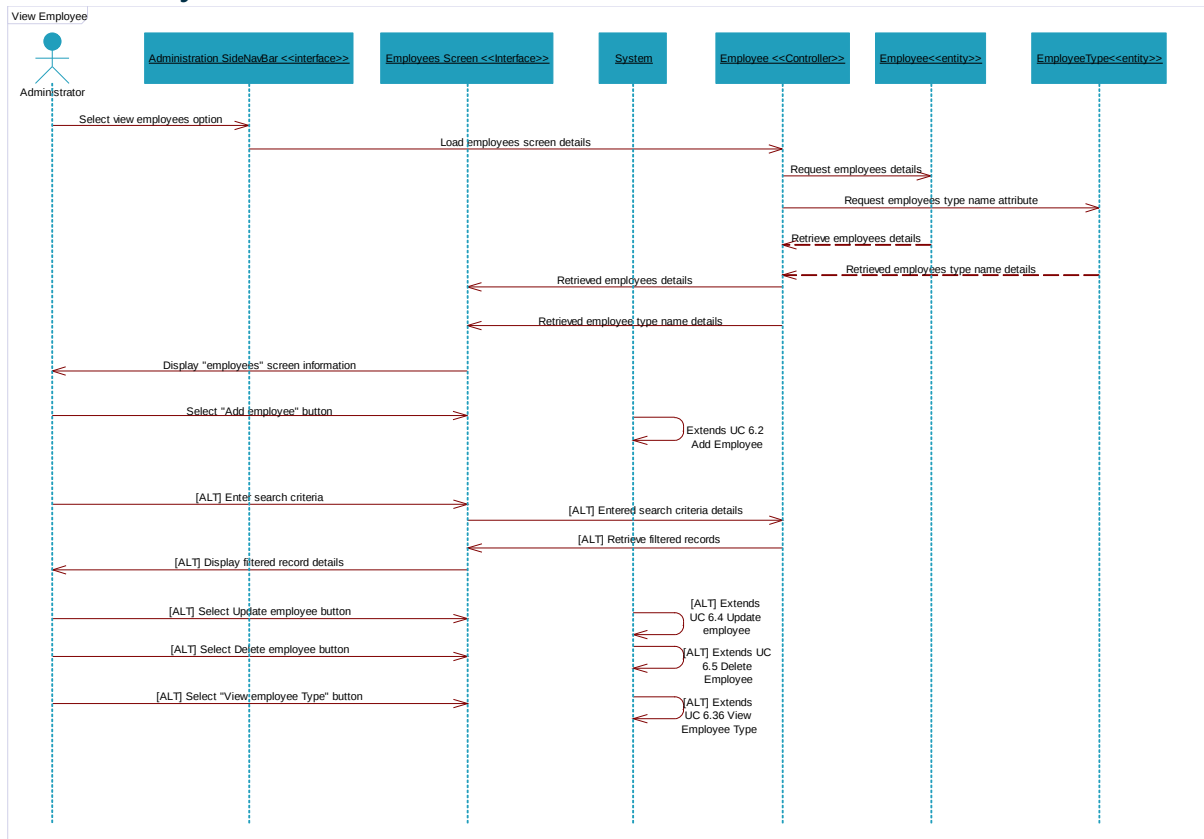
Figure 30: 6.1- View Employee Sequence Diagram
