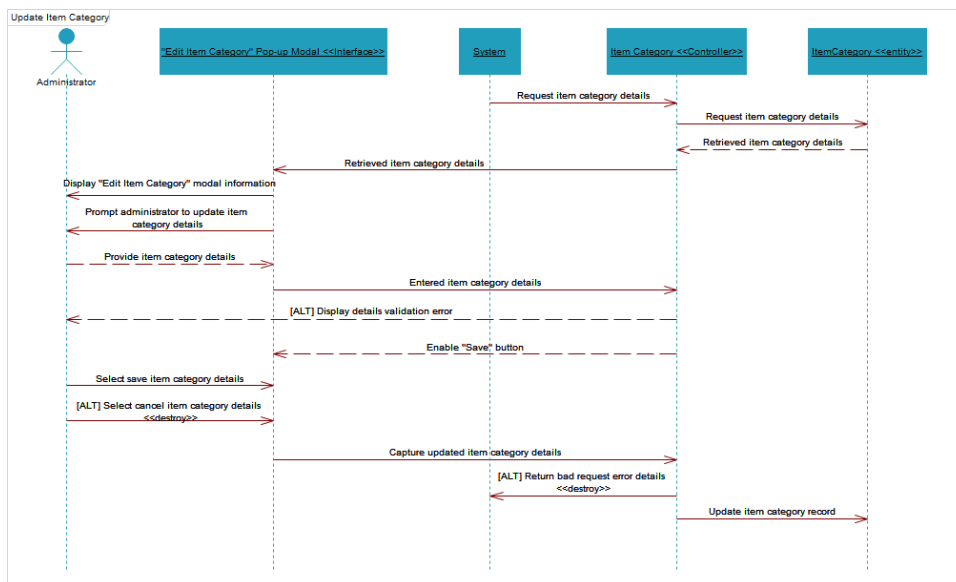
Figure 67: 7.11-Update Item Category Sequence Diagram
