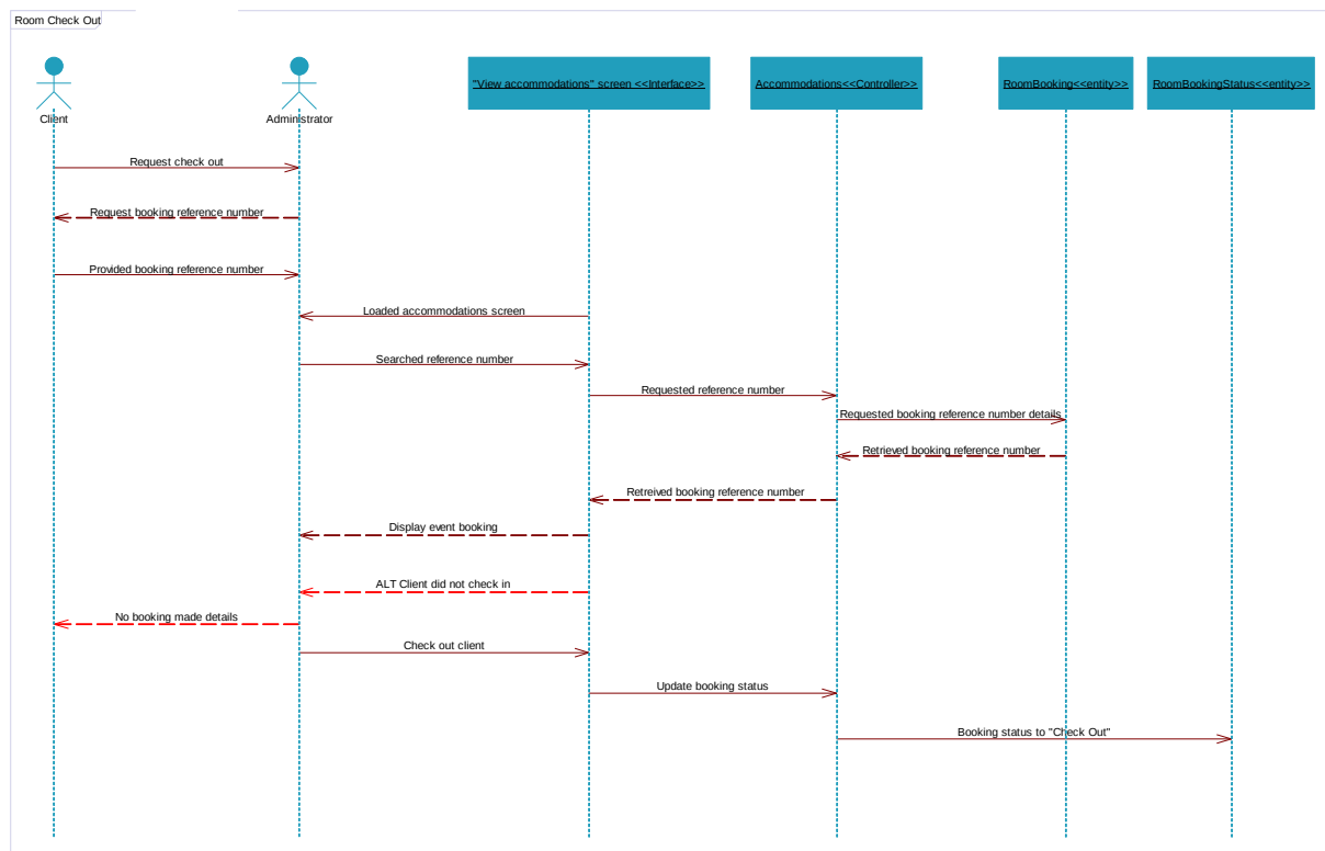
Figure 40:6.11-Room Check-Out Sequence Diagram
