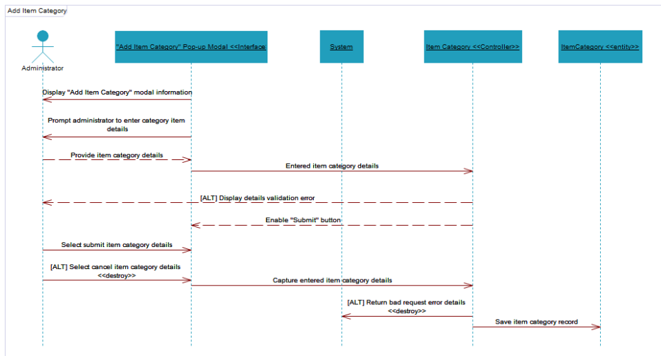
Figure 66:7.10- Add Item Category Sequence Diagram
