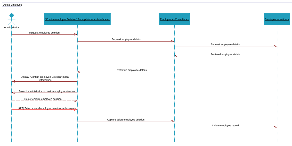
Figure 33: 6.4- Delete Employee Sequence Diagram
