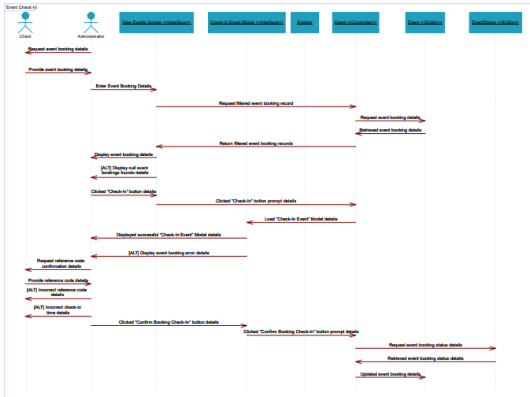
Figure 50: 6.21-Event Check-In Sequence Diagram
