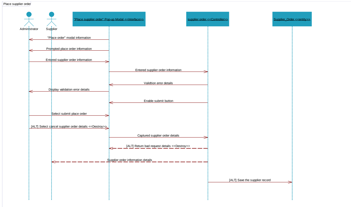
Figure 74:7.18-Place Supplier Order Sequence Diagram
