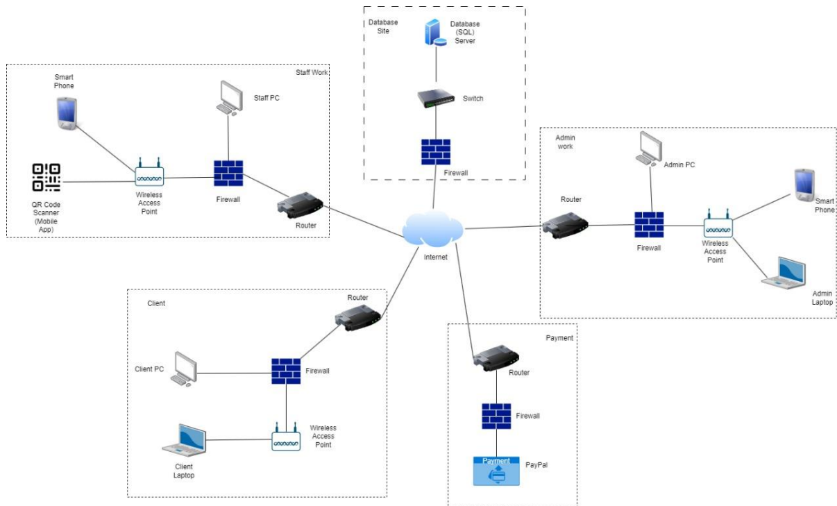
Figure 1: Network layout for HydroTech system
