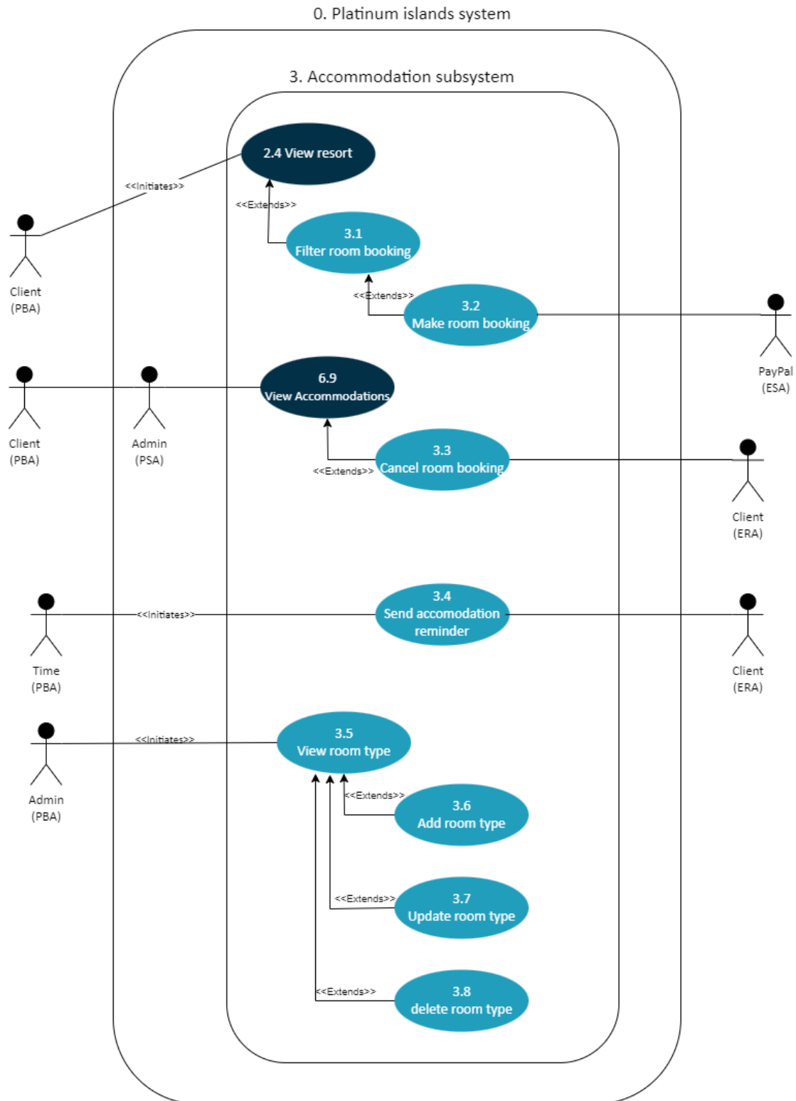
Figure 3:Accommodation Subsystem UCD
