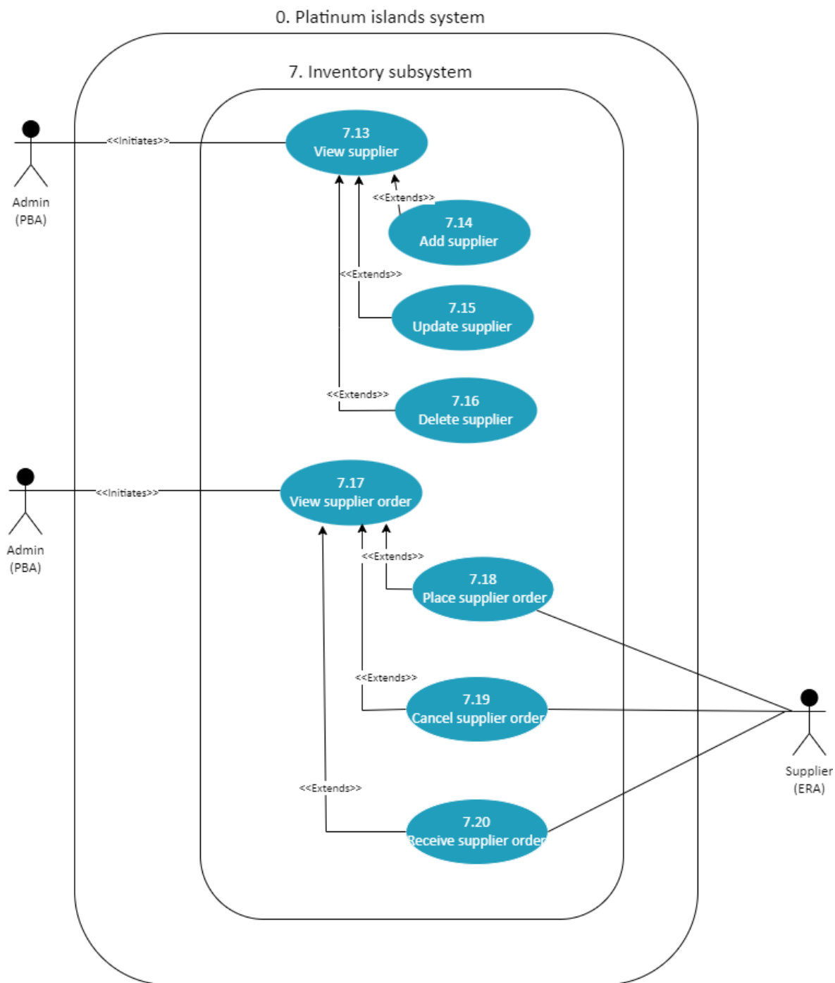
Figure 9: Inventory Subsystem UCD Part 2
