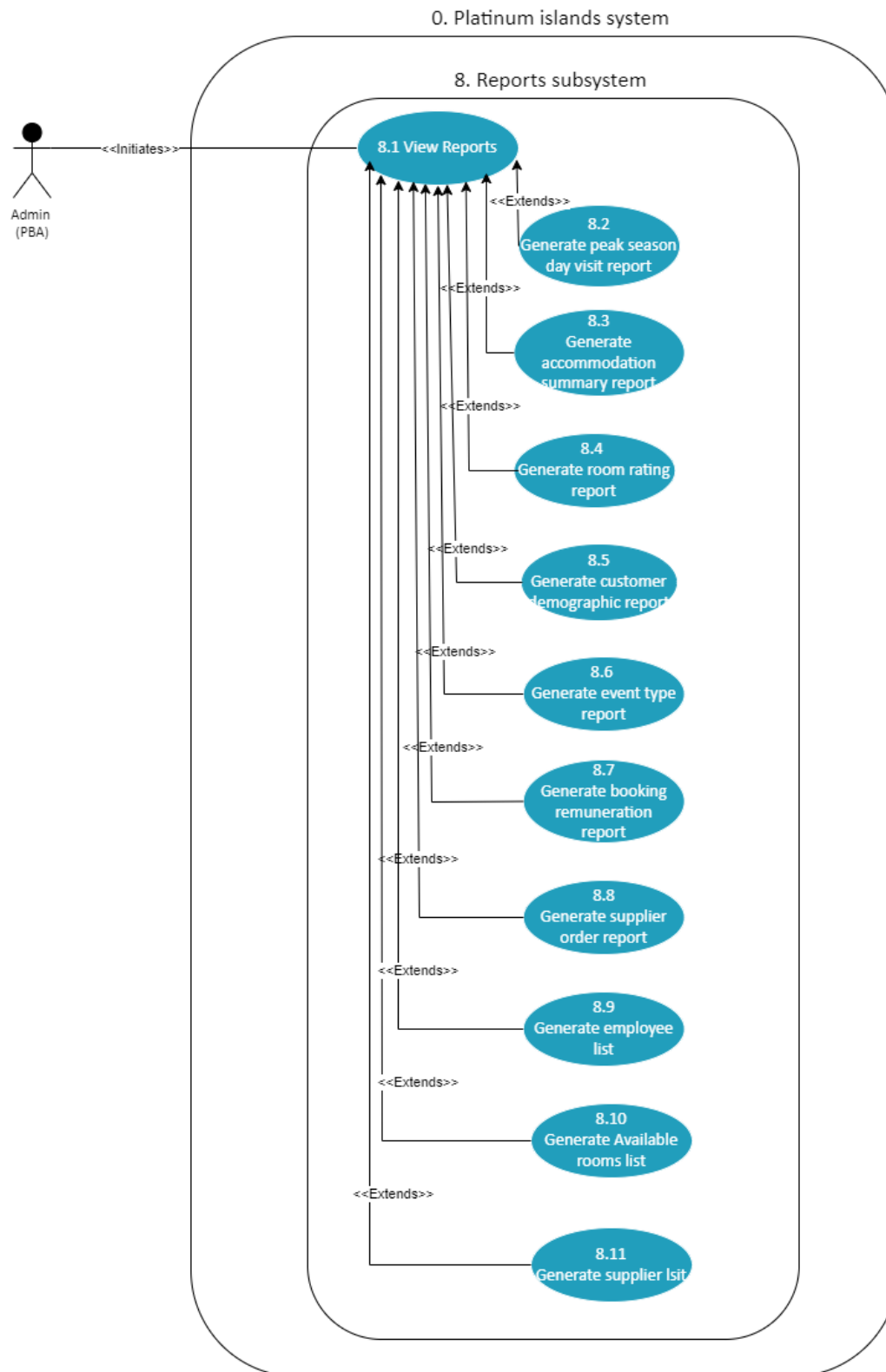
Figure 10:Report Subsystem UCD
