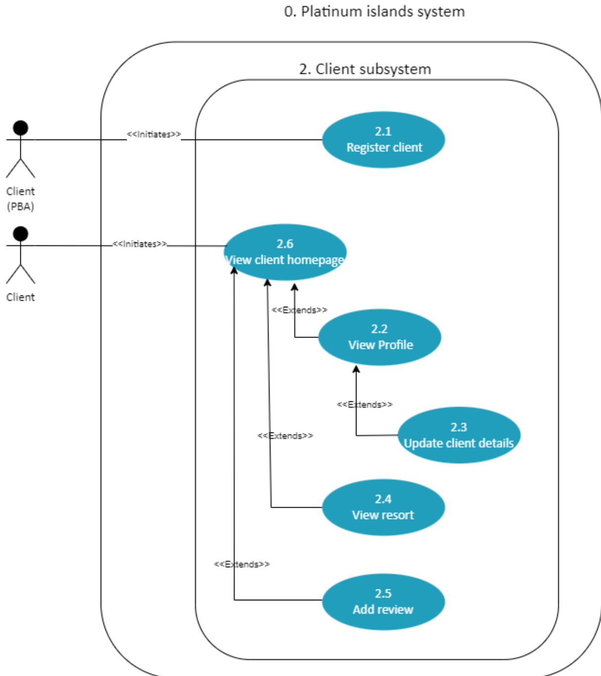
Figure 2: Client Subsystem UCD
