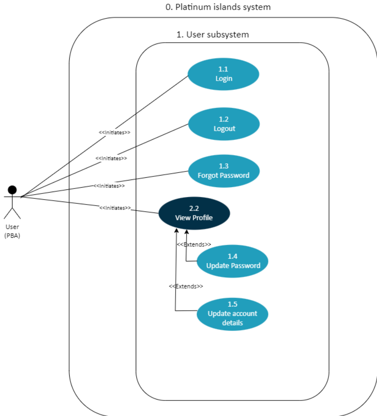
Figure 1: User Subsystem UCD
