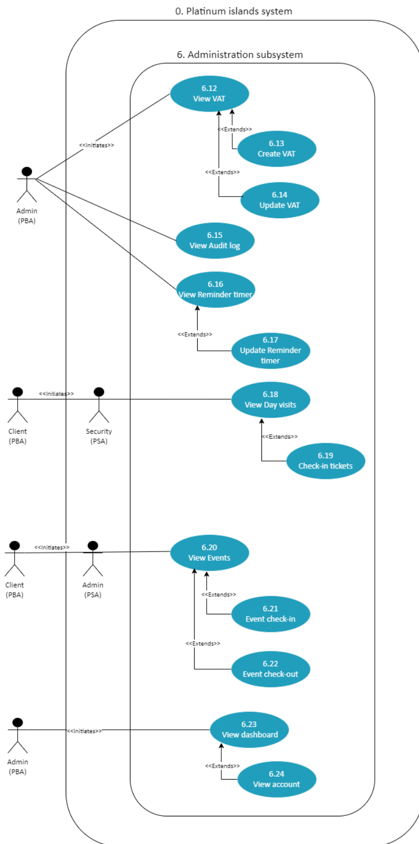
Figure 7:Administration Subsystem UCD Part 2
