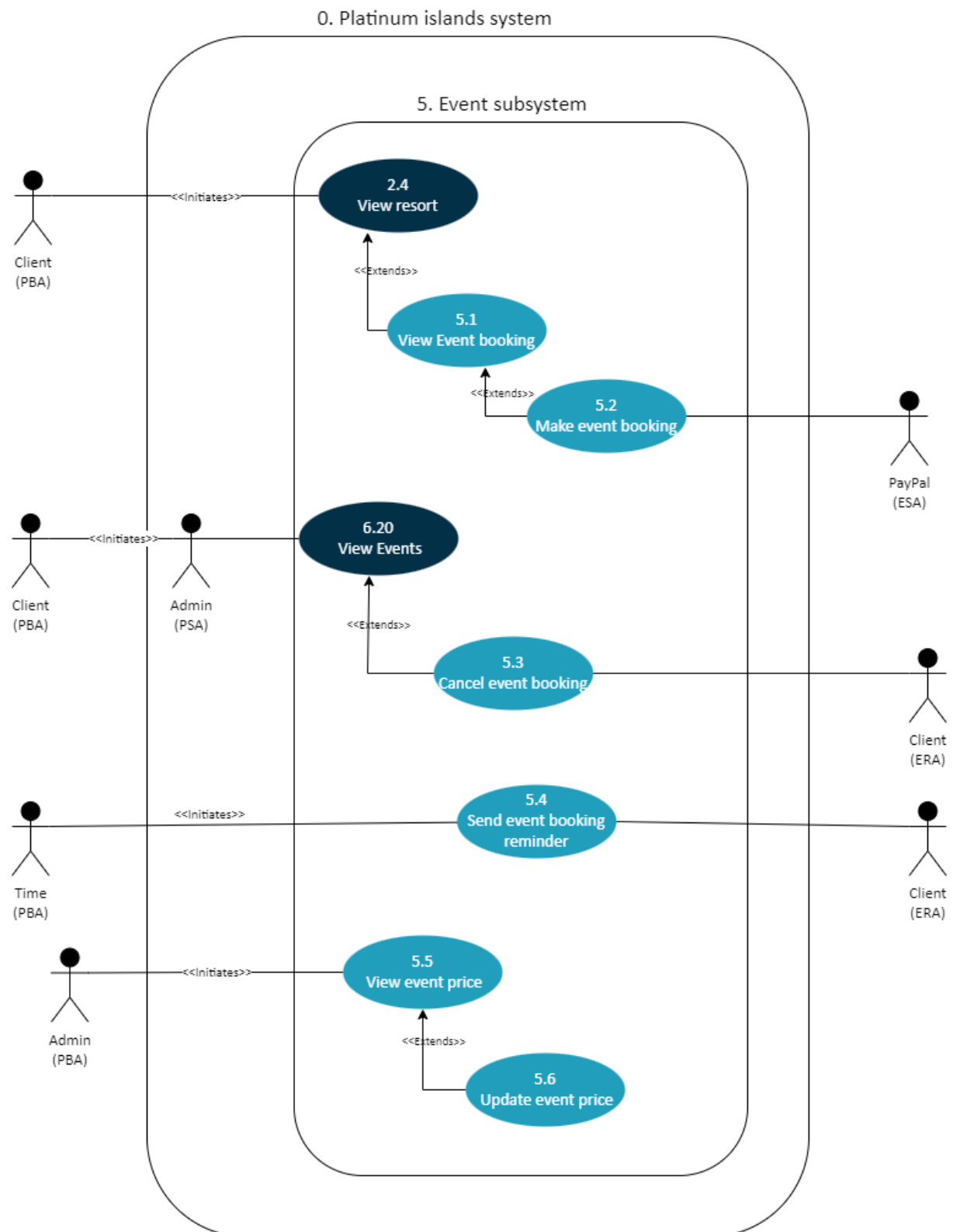
Figure 5: Event Subsystem UCD
