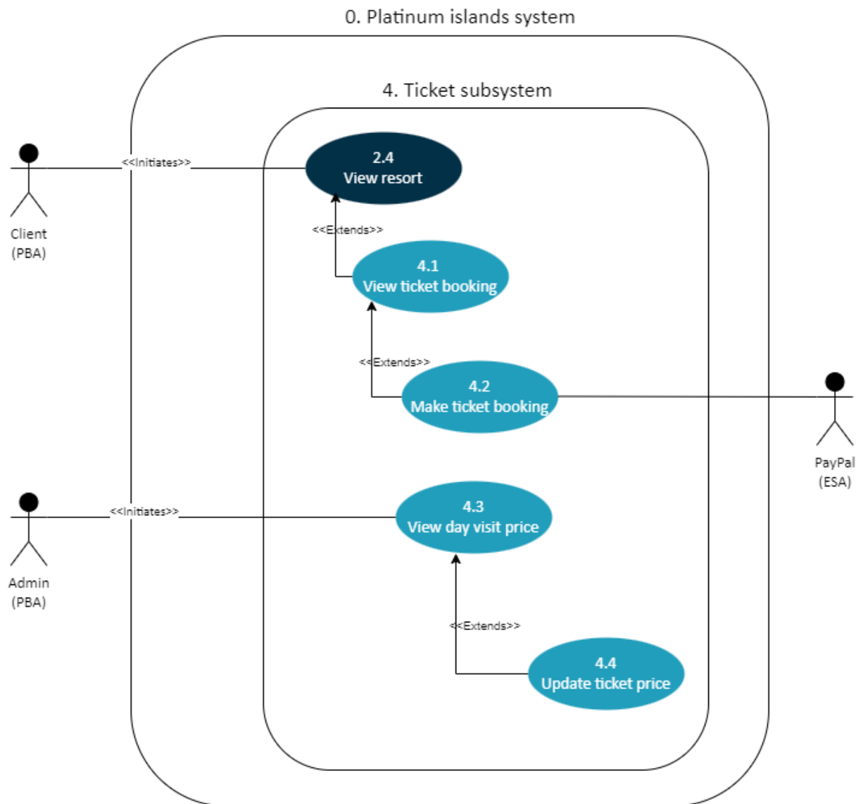
Figure 4: Ticket Subsystem UCD
