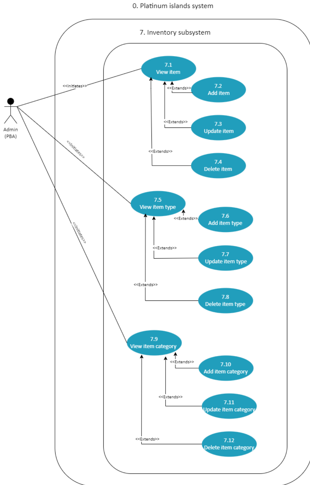
Figure 8:Inventory Subsystem UCD Part 1
