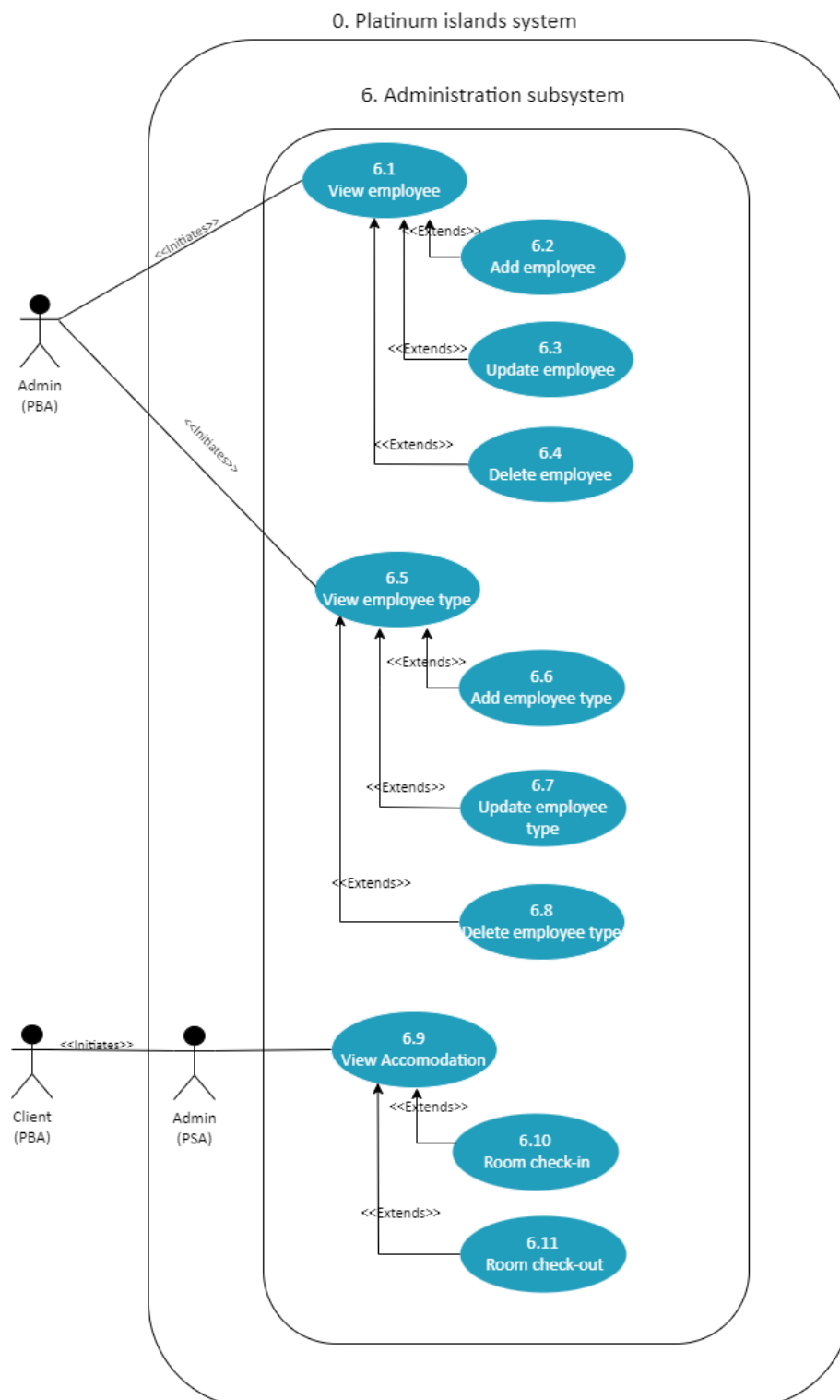
Figure 6:Administration Subsystem UCD Part 1
